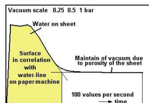
FRET DYNAMIC DRAINAGE CURVE
